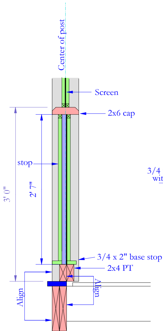
Wall Section
